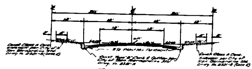
TYPICAL SECTION VINE ST., ROSALIND AVE., BURN EY ST., BELDEN ST.
